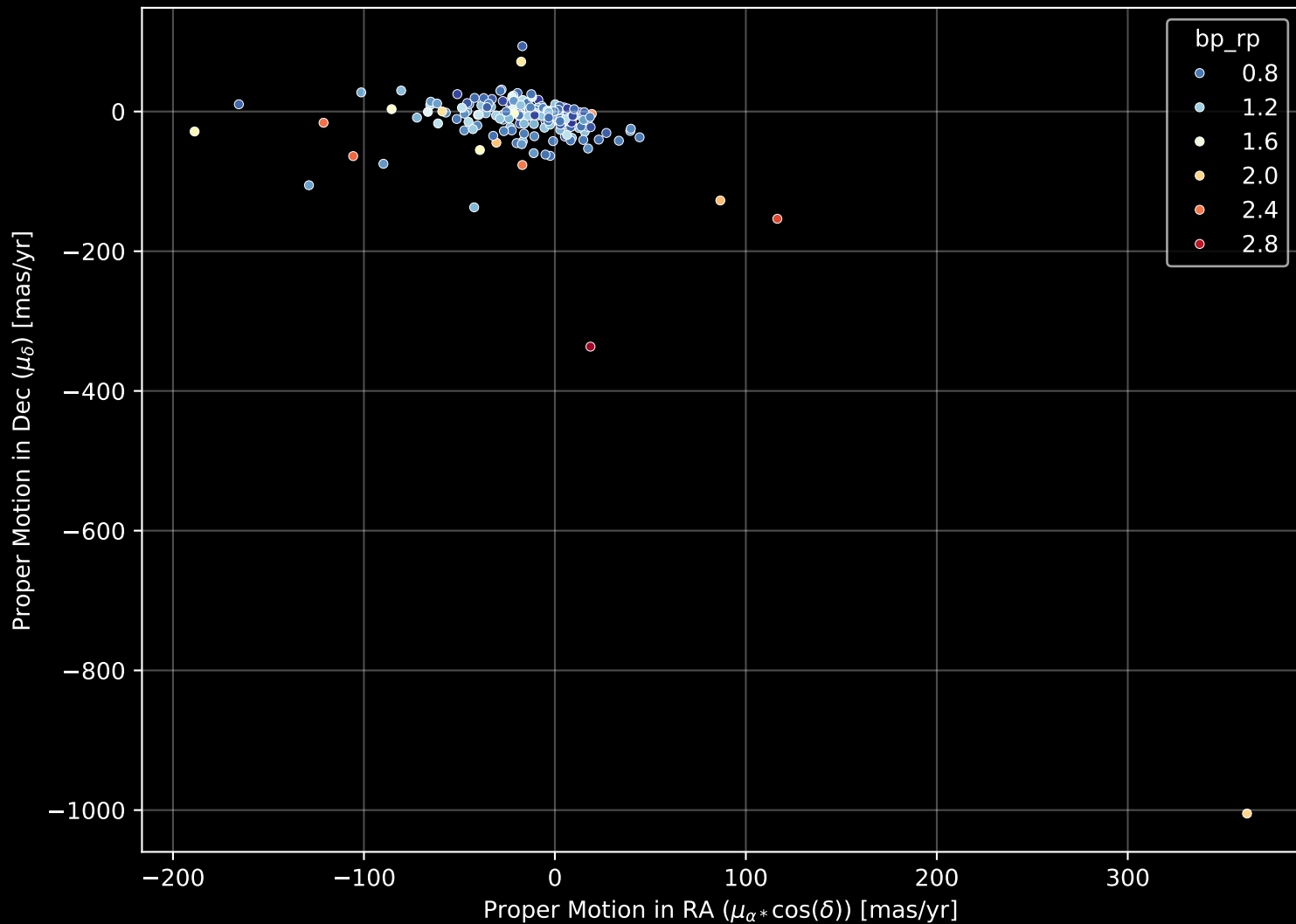
APOGEE DR17 Field: [073+72_MGA] Proper Motion Diagram (n= 192)
