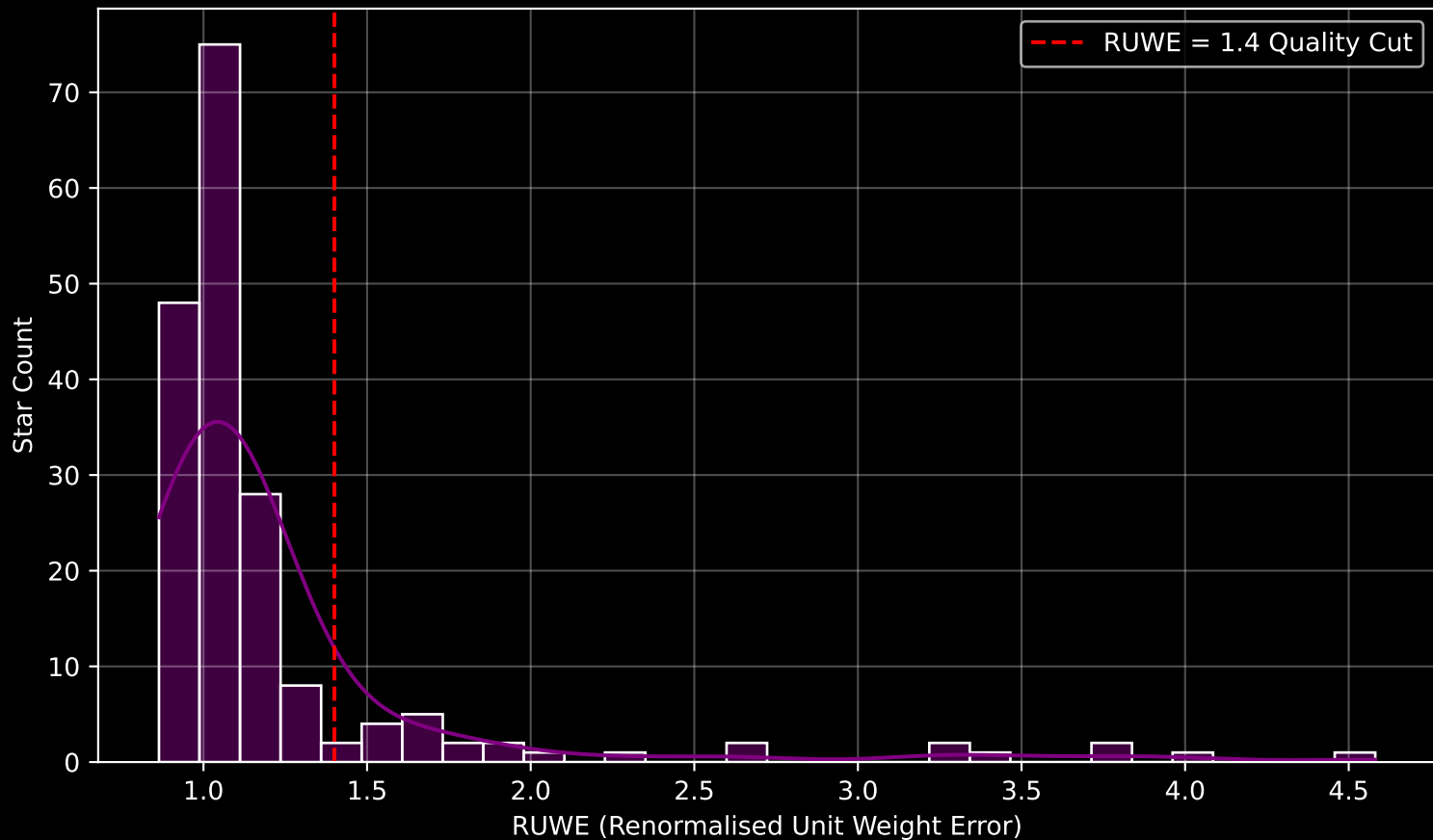
GAPOGEE DR17 Field [073+72_MGA] RUWE Distribution (n= 185)
