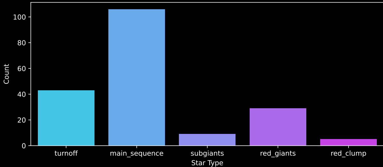
APOGEE DR17 Field: [073+72_MGA] Count plot of Star Type
