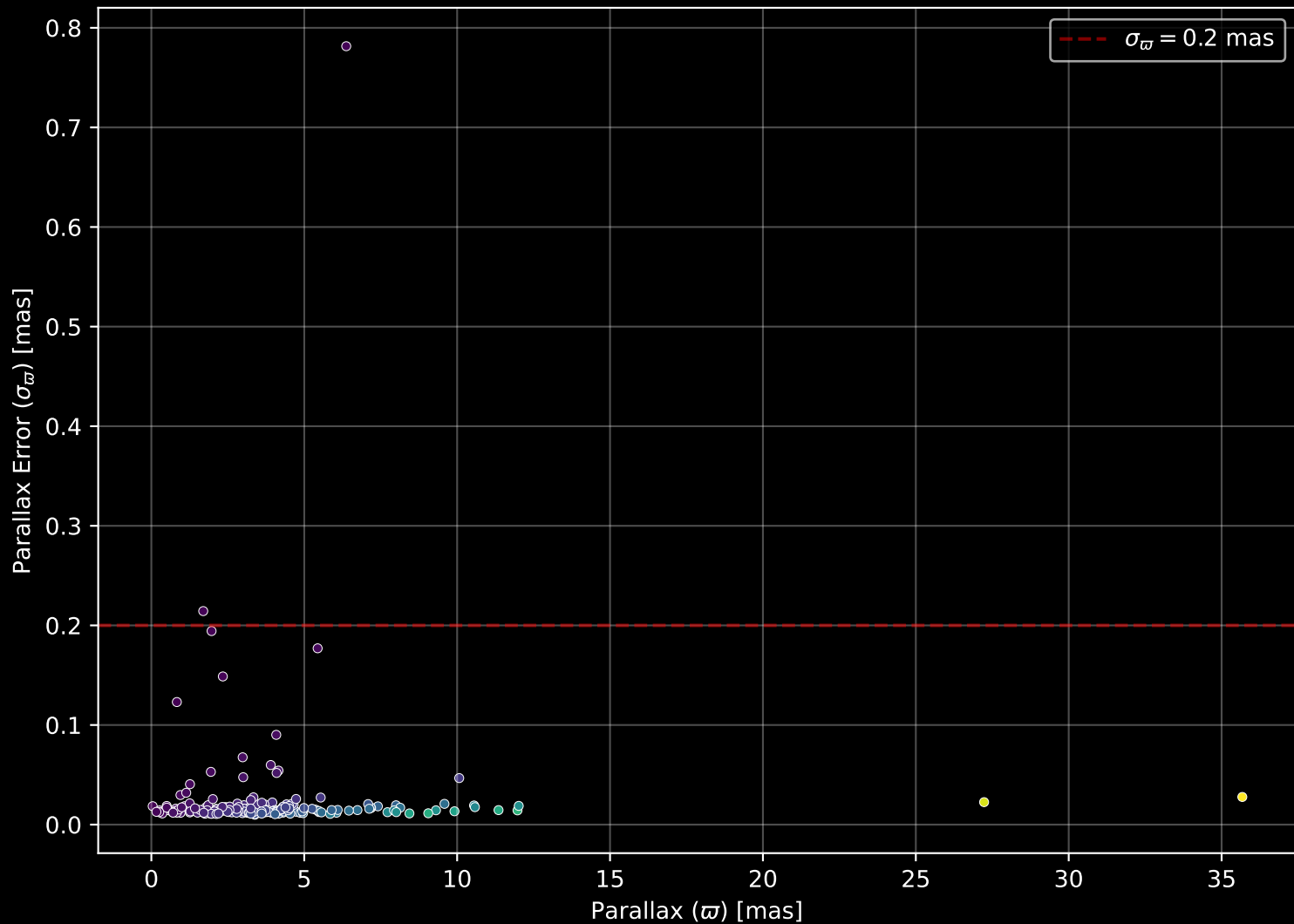
APOGEE DR17 Field: [073+72_MGA] Parallax Quality (n= 192)
