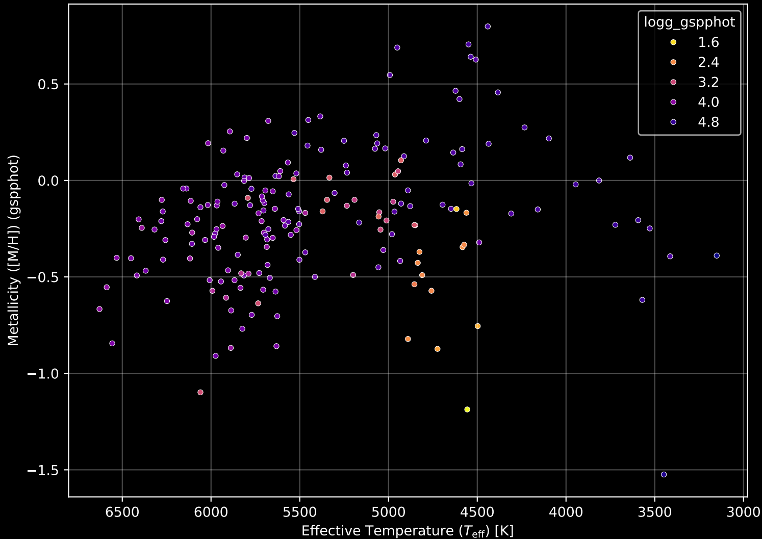
APOGEE DR17 Field: [073+72_MGA] Stellar Population Parameters (n= 192)
