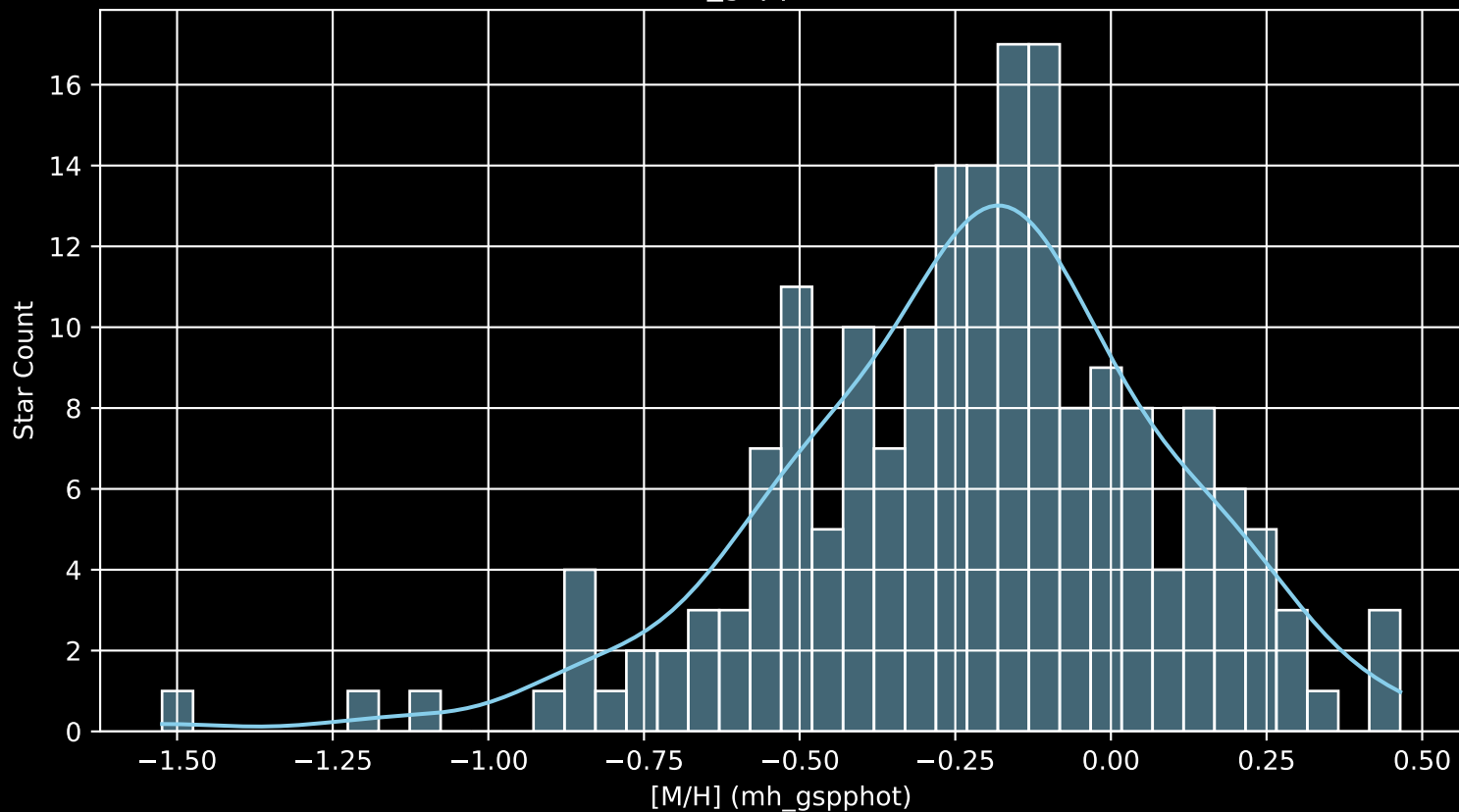
APOGEE DR17 Field: [073+72_MGA [M/H] (mh_gspphot) (n= 186)
